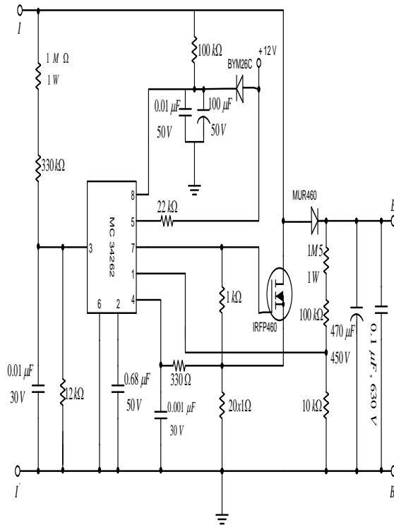
Figure 4. Power factor correction circuit
