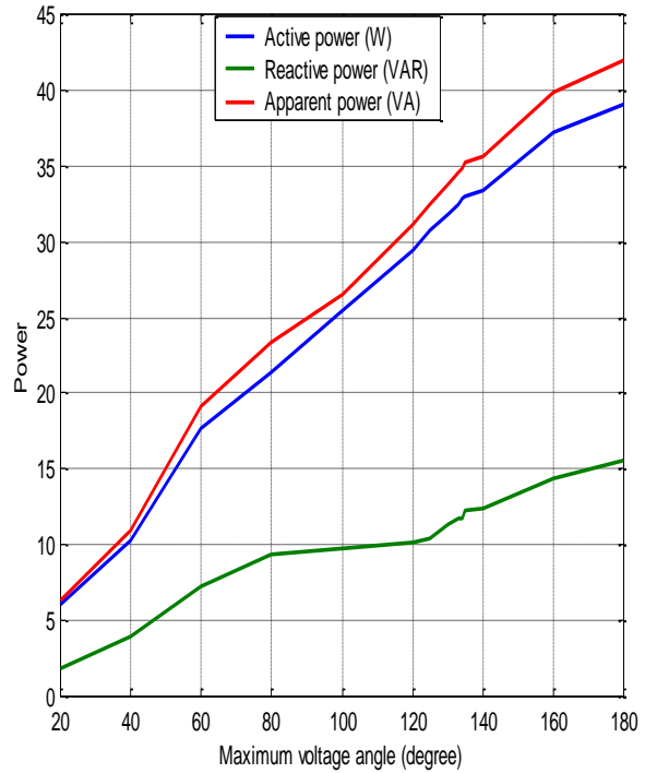
Figure 13. Effect of maximum voltage angle on the AC power
