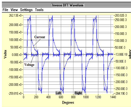
(c) Maximum voltage angle at 60^{\circ}
