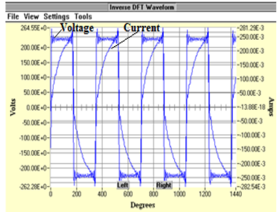
(g) Maximum voltage angle at 180^{\circ}
