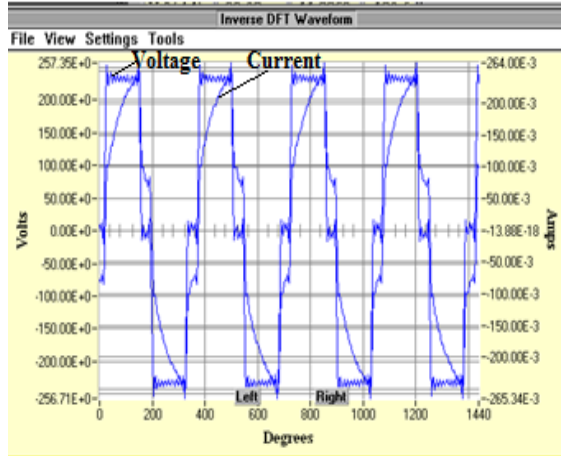
(f) Maximum voltage angle at 135^{\circ}
