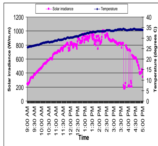
Figure 8. Solar irradiance and temperature on 28 th February 2014
