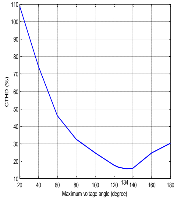
Figure 14. Effect of maximum voltage angle on current total harmonic distortion (CTHD)
