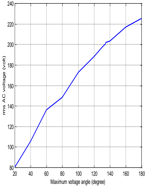
Figure 11. Effect of maximum voltage angle on the AC voltage
