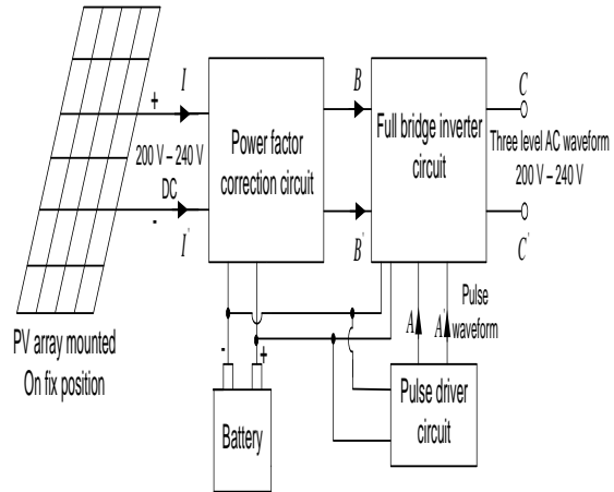
Figure 2. Realized single phase TPVI system
