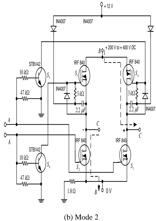
Figure 5. Two operation modes of proposed TPVI
