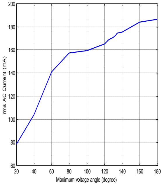
Figure 12. Effect of maximum voltage angle on the AC current
