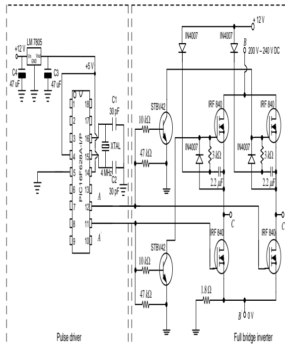
Figure 3. Pulse driver and full bridge inverter circuit
