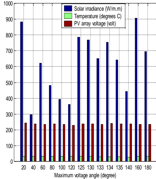
Figure 9. Condition of solar irradiance, temperature and PV array voltage varying maximum voltage angle
