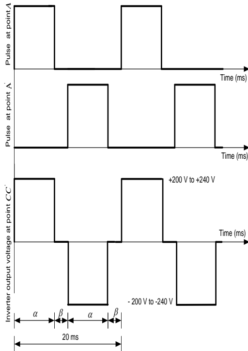
Figure 6. Pulse and three-level output waveform of the TPVI
